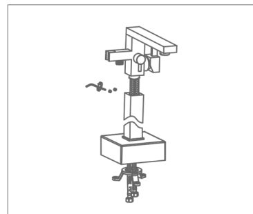
2. Tighten the flexible lines to the head. Slide the head and lines through the square body. Fix the head to the body with set screws.
