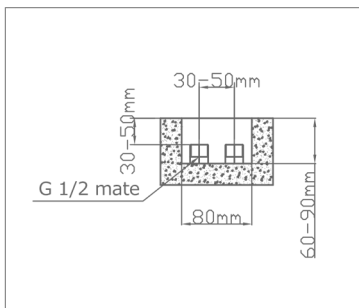
3. Dimensions of the void in the floor for the water inlets.
