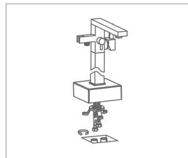
4. Slide the cover plate over the body and tighten the flexible lines to the water supply inlet.
