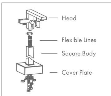
1. Diagram of the faucet parts.
