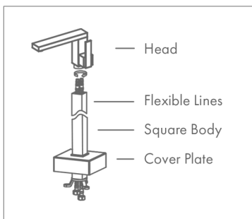
1. Diagram of the faucet parts.
